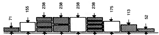
⑫ Interrelationship between brick/block height dimensions → ⑪
